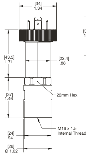
F16 Fitting Shown
