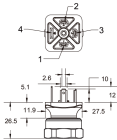
DA - EN17530-803 Form A (DIN 43650 Form A)
