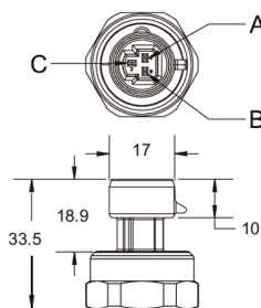
GN-Metri-Pack®
