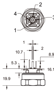
DC - EN17530-803 Form C (DIN 43650 Form C)
